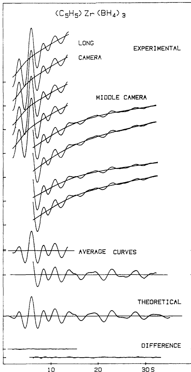
Figure 3. Intensity curves for cyclopentadienylzirconium tetrahydroborate. The s^4I_e experimental curves are shown magnified 5 times with respect to the backgrounds on which they are superimposed. The average curves are s^4I_e - bkgd . The theoretical and difference curves are for the tridentate model of Table I.
